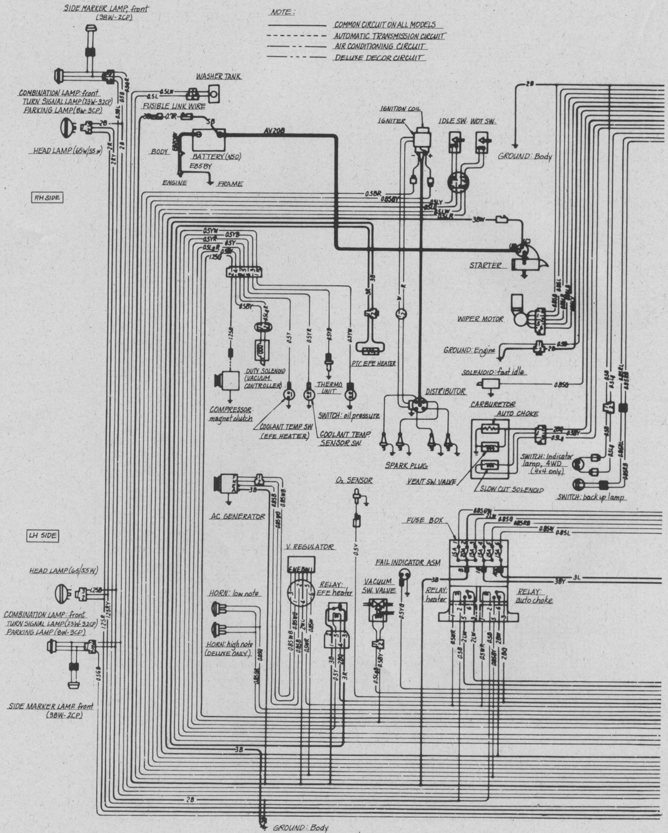
Fig. 13.89 Wiring diagram (Series 12, California models) (1 of 2)
