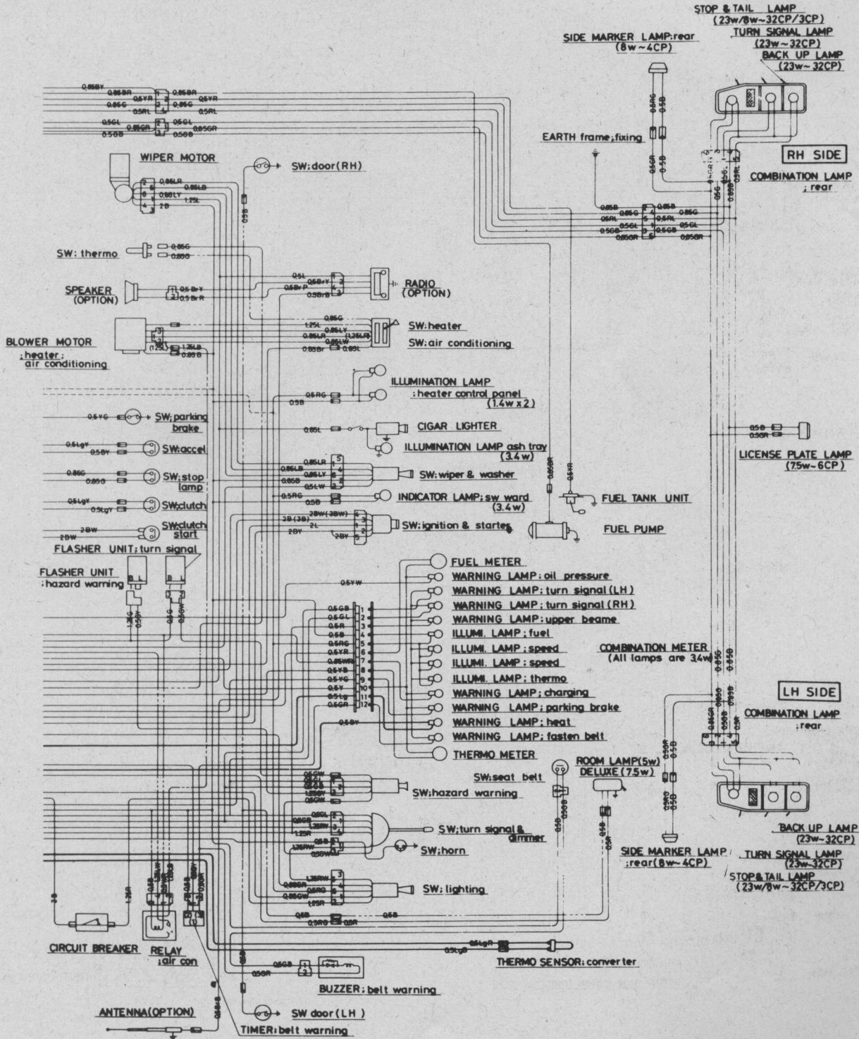
Fig. 13.84 Wiring diagram (Series 9 and 10) (2 of 2)
