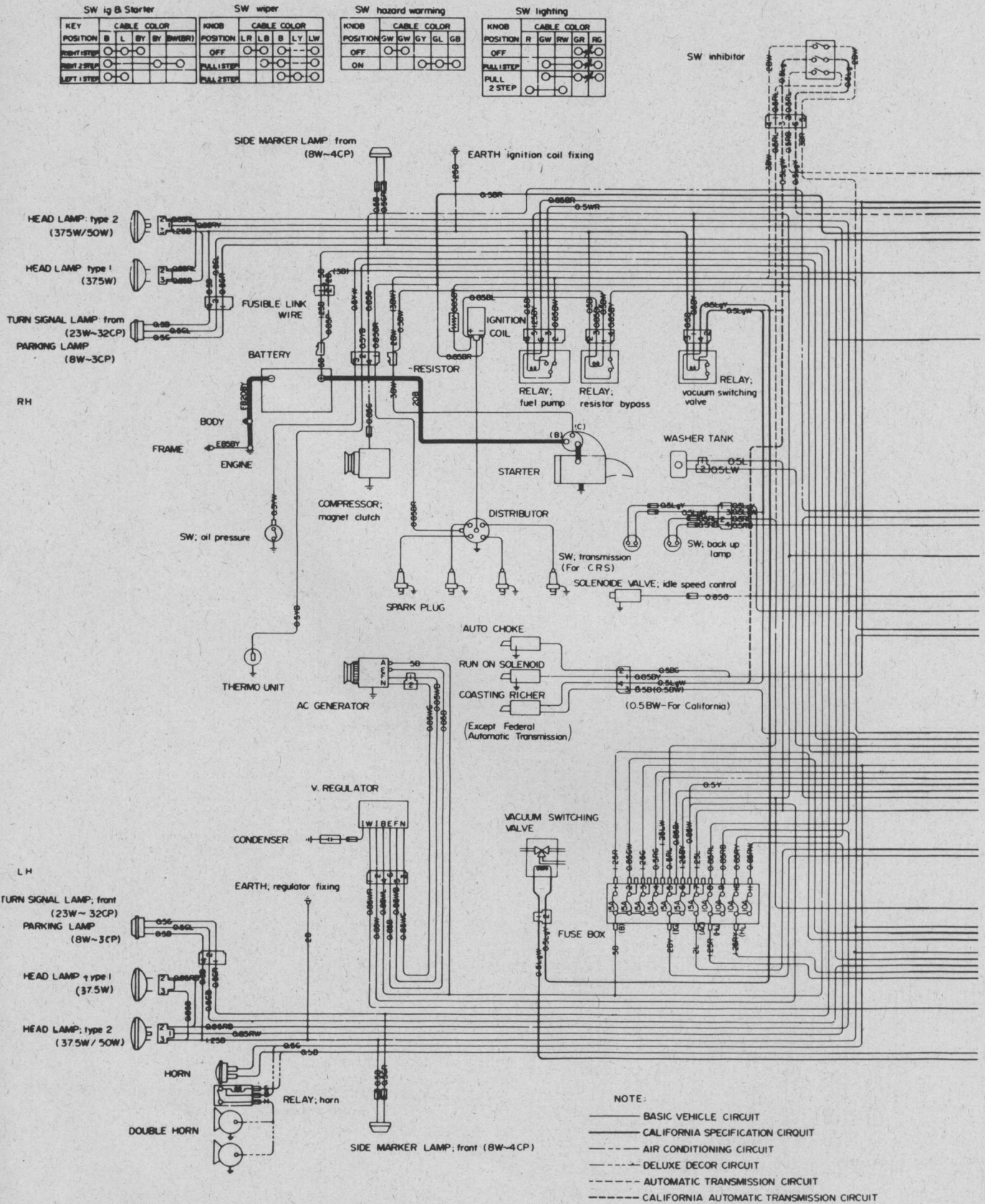
Fig. 10.53. Wiring diagram - Series 6 models
