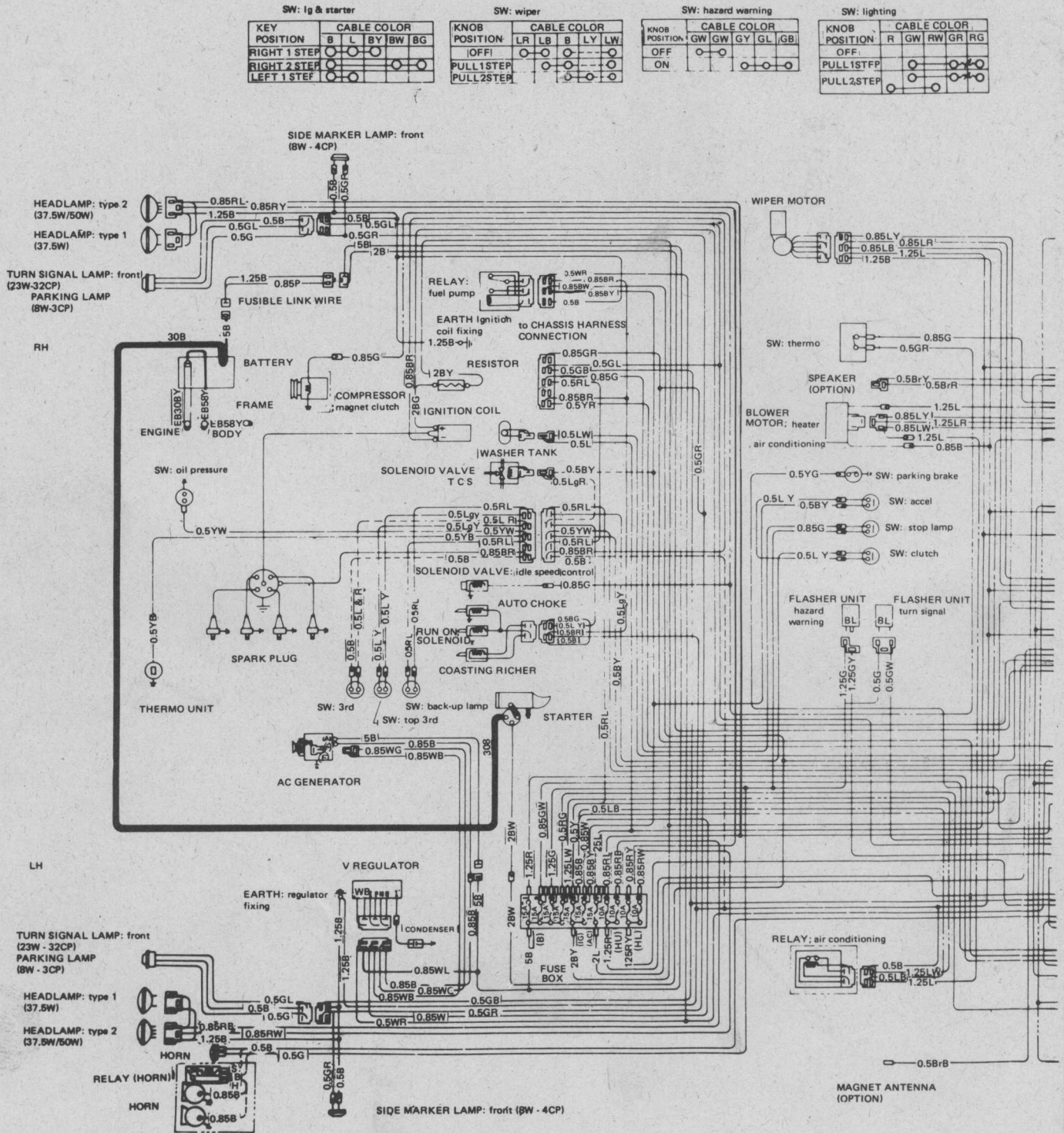
Fig. 10.51. Wiring diagram Series 4 model
